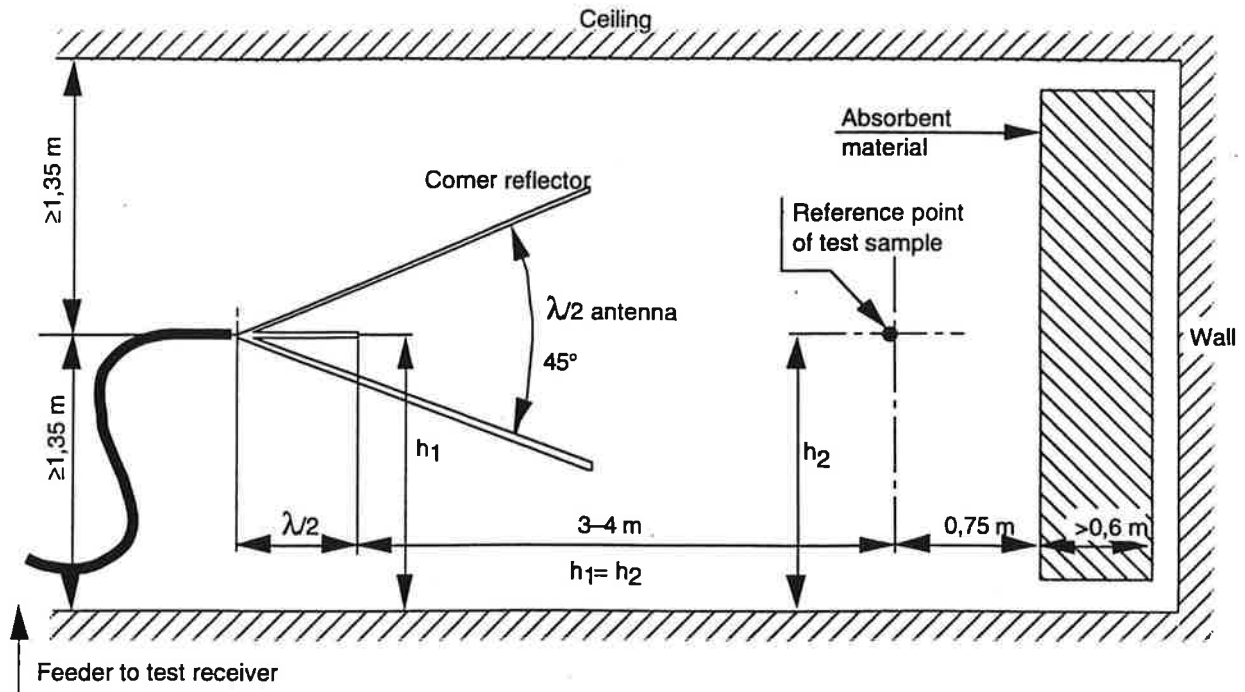
Fig. 1.2 Indoor site arrangement (shown for horizontal polarisation)
