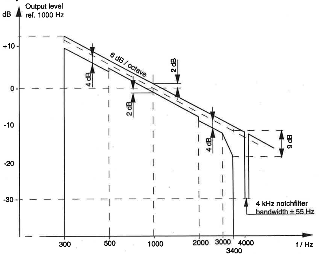
Figure 3. Audio frequency response of the combination receiver line interface
