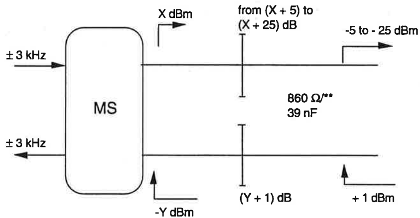
Figure 6. Measuring levels for connecting a 4-wire equipment to a mobile station
