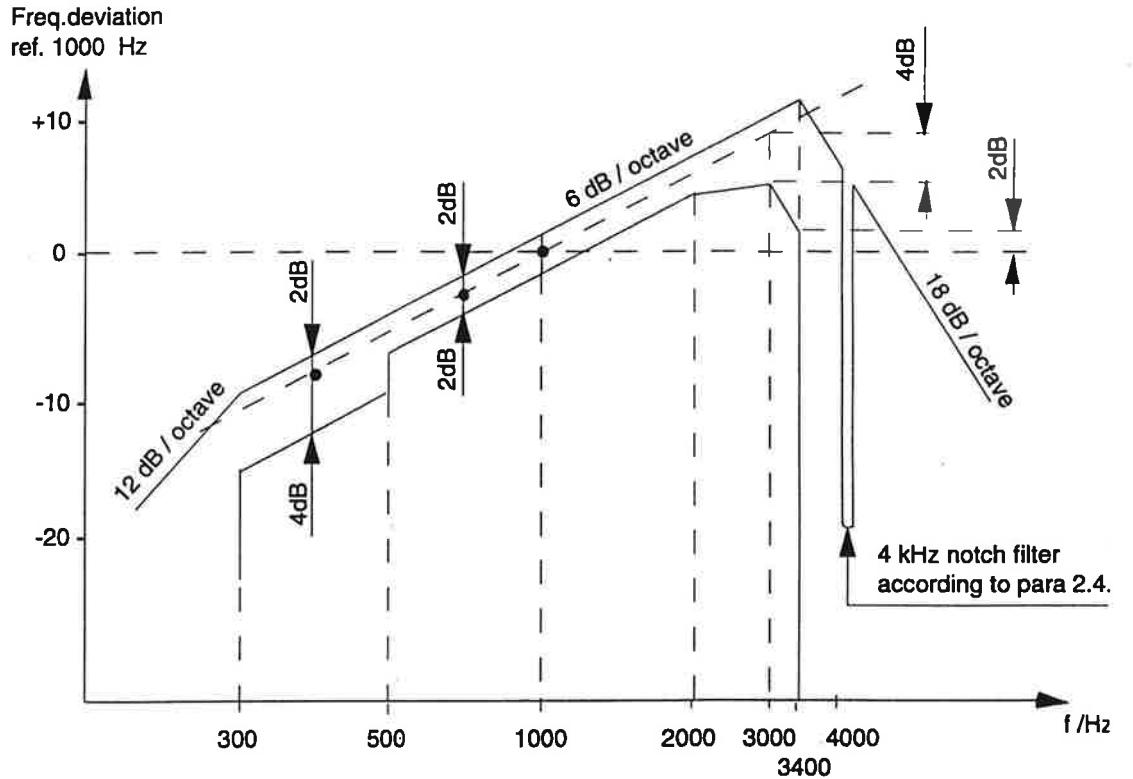
Figure 2. Audio frequency response of the combination transmitter line interface
