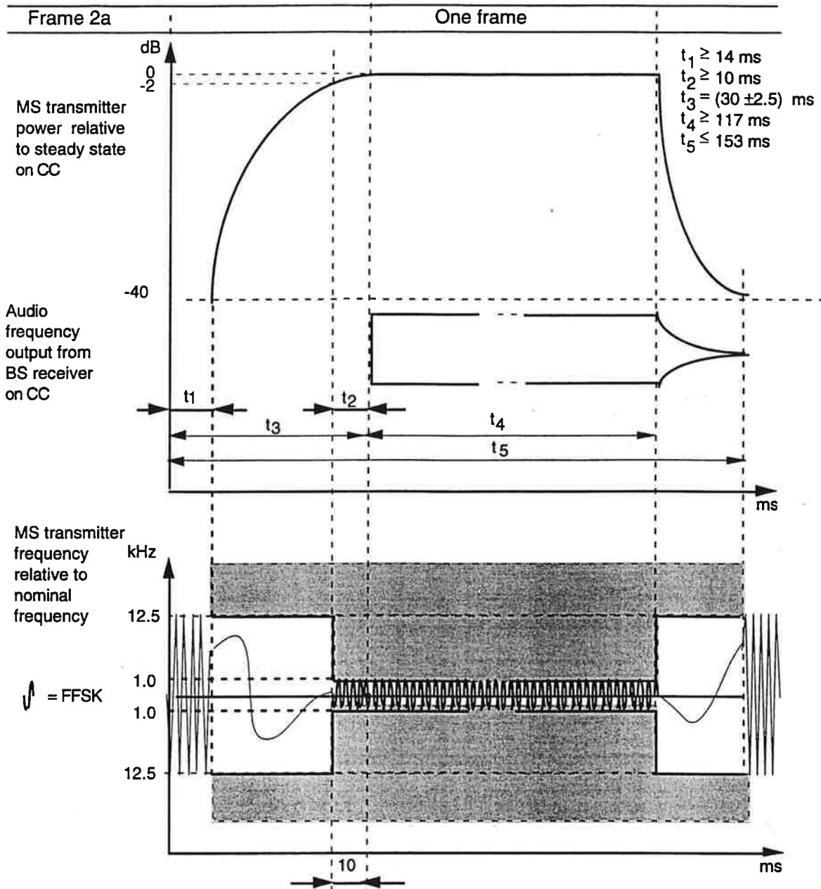
Fig. 6.3 Transmitter frequency transient behaviour, start up and decay times
