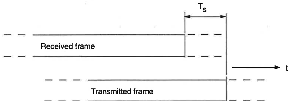
Fig 5.15 Time skew
